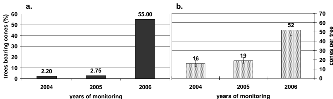
Figure 1 – a. Percentage of mature trees bearing cones per sampling plot (100m 2 ) and b. average number of cones per tree, during the years of study.
